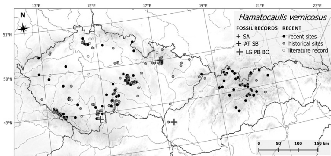
Fig. 5. – Distribution of Hamatocaulis vernicosus in the Czech and Slovak Republics based on fossil, herbarium and published data. See Methods for the abbreviations of periods.
