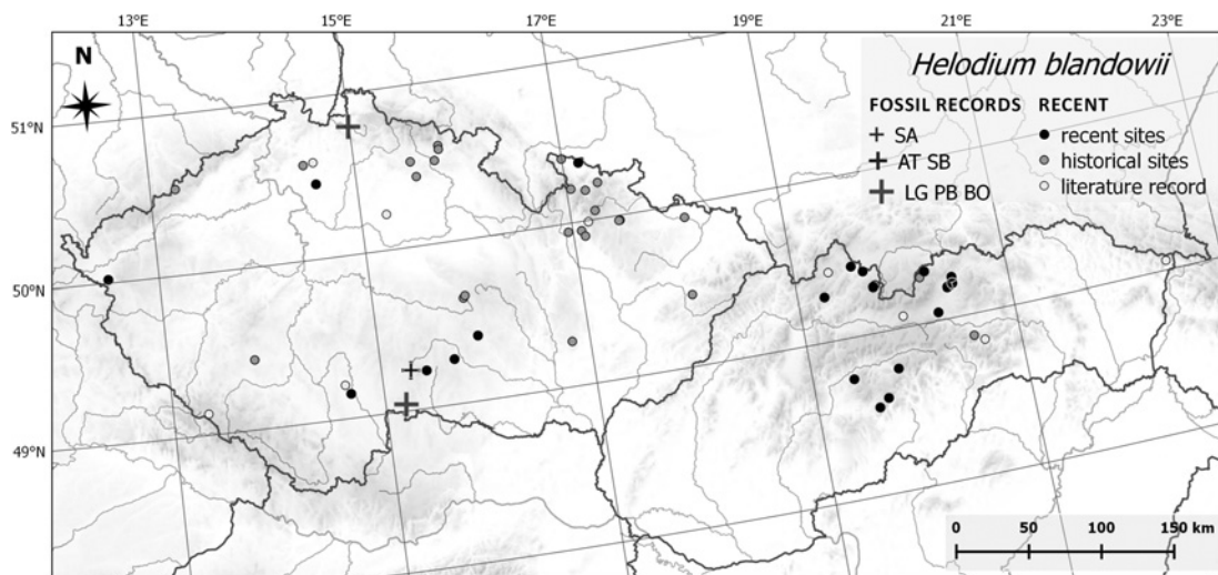
Fig. 6. – Distribution of Helodium blandowii in the Czech and Slovak Republics based on fossil, herbarium and published data. See Methods for the abbreviations of periods.
