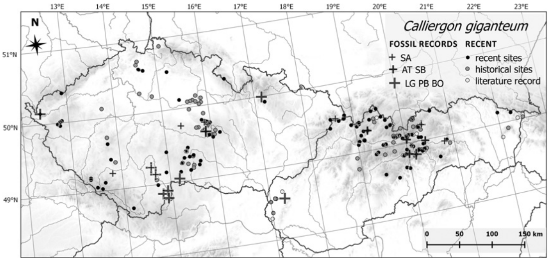
Fig. 3. – Distribution of Calliergon giganteum in the Czech and Slovak Republics based on fossil, herbarium and published data. See Methods for the abbreviations of periods.
