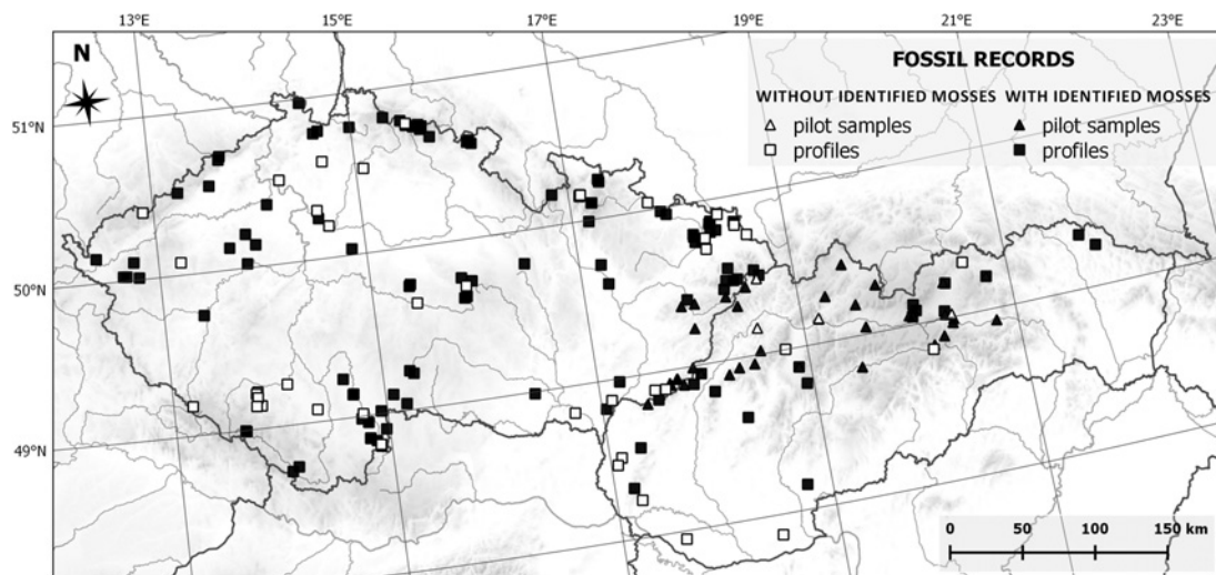
Fig. 2. – Distribution of macrofossil data with and without bryophytes.
