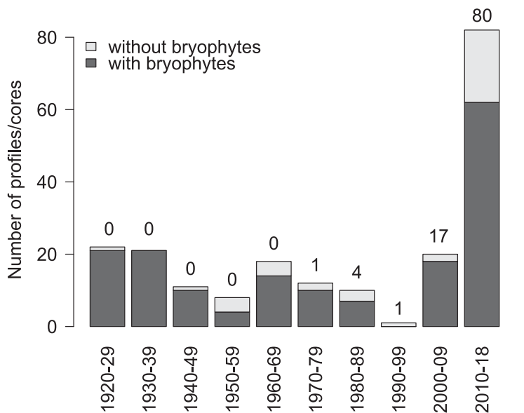
Fig. 1. – Number of profiles and cores in particular periods with (grey colour) and without (white colour) identified bryophytes. The number above the bars indicates the number of radiocarbon-dated profiles.
