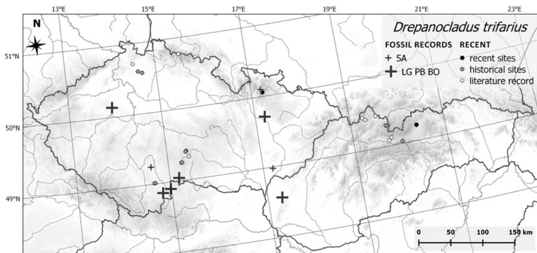
Fig. 4. – Distribution of Drepanocladus trifarius in the Czech and Slovak Republics based on fossil, herbarium and published data. See Methods for the abbreviations of periods.
