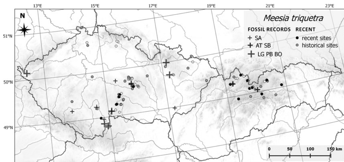
Fig. 7. – Distribution of Meesia triquetra in the Czech and Slovak Republics based on fossil, herbarium and published data. See Methods for the abbreviations of periods.
