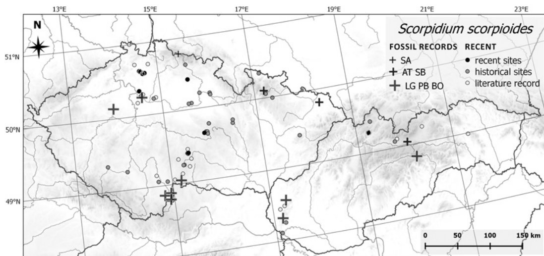
Fig. 9. – Distribution of Scorpidium scorpioides in the Czech and Slovak Republics based on fossil, herbarium and published data. See Methods for the abbreviations of periods.
