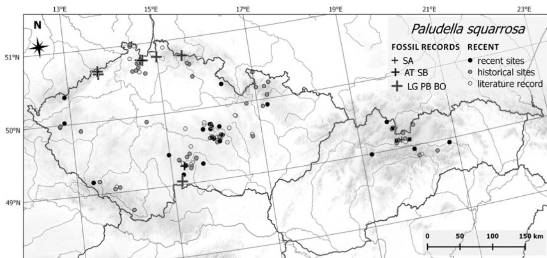
Fig. 8. – Distribution of Paludella squarrosa in the Czech and Slovak Republics based on fossil, herbarium and published data. See Methods for the abbreviations of periods.
