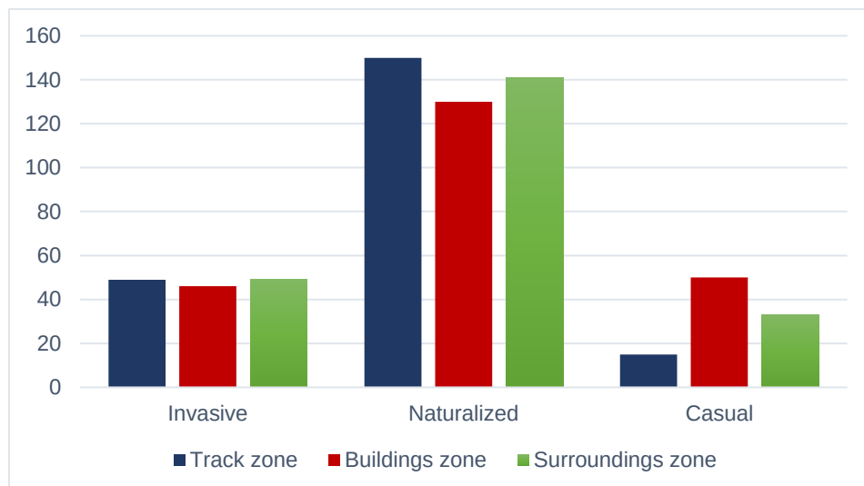
Supplementary Fig. S1. (A) The number of aliens in examined zones
