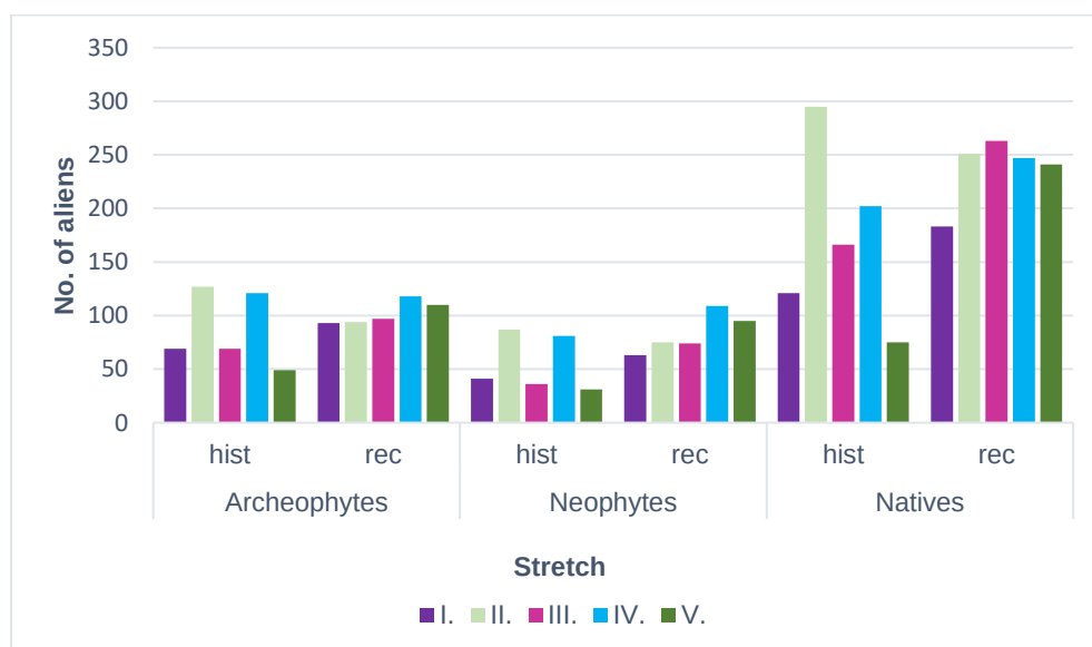
Supplementary Fig. S1. (B) The number of recent (rec) and historical (hist) alien taxa divided according to the residence time.
