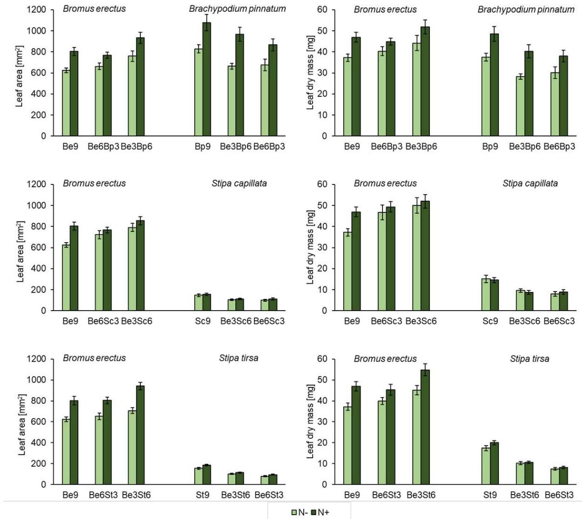
Supplementary Fig. S5. – First year performance in terms of the leaf area (left) and leaf dry mass (right) per individual of Bromus erectus in combination with Brachypodium pinnatum (above), Stipa capillata (middle) and S. tirsia (below). The different coloured bars (mean + SE) represent the different species compositions (9, 6:3, 3:6) in the different nutrient conditions. Using two-way ANOVA for testing mean differences (see Table S4).
